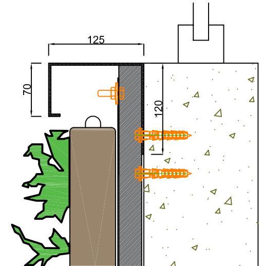
Detail 2 1:5
