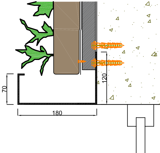
Detail 3 1:5
