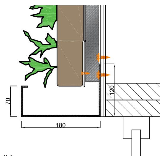
Detail 3 1:5
