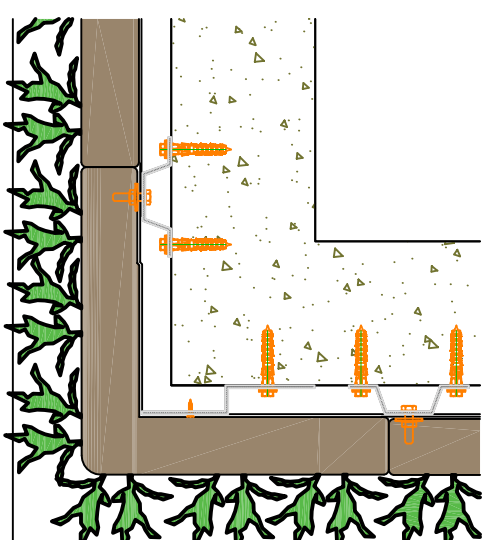
Detail 1 1:8
